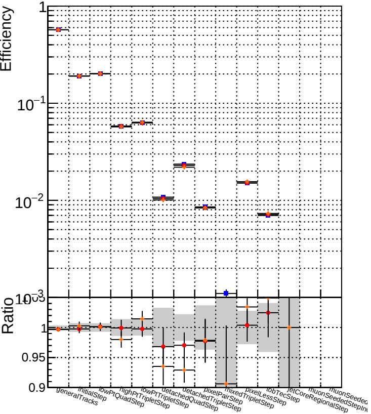
DQM_TT_mkFit_ORIG DQM_TT_mkFit_MODIF /data2/legianni/newRel-PR129/sta/CMSSW_13_2_0_pre3/src/DQM_TT_MODIFok
