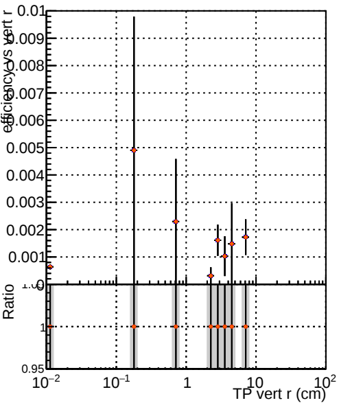
Efficiency vs TP vert r (cm) Legend: DQM_TT_mkFit_ORIG DQM_TT_mkFit_MODIF /data2/legianni/newRel-PR129/sta/CMSSW_13_2_0_pre3/src/DQM_TT_MODIFok
