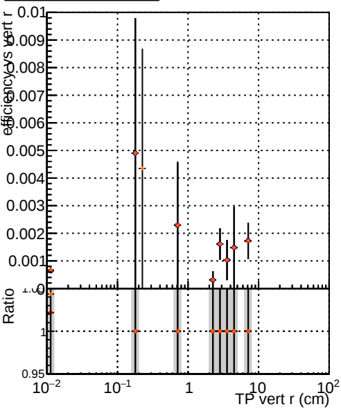
Efficiency vs vertpos Legend: DQM_TT_mkFit_ORIG DQM_TT_mkFit_MODIF /data2/legianni/newRel-PR129/sta/CMSSW_13_2_0_pre3/src/DQM_TT_MODIFok
