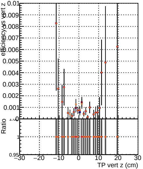
Efficiency vs vertpos Legend: DQM_TT_mkFit_ORIG DQM_TT_mkFit_MODIF /data2/legianni/newRel-PR129/sta/CMSSW_13_2_0_pre3/src/DQM_TT_MODIFok
