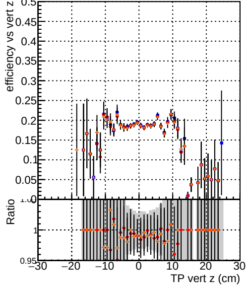
Efficiency vs. TP vert z (cm) Legend: - DQM_TT_mkFit_ORIG (blue circles) - DQM_TT_mkFit_MODIF (red circles) - /data2/legianni/newRel-PR129/sta/CMSSW_13_2_0_pre3/src/DQM_TT_MODIFok (orange circles)
