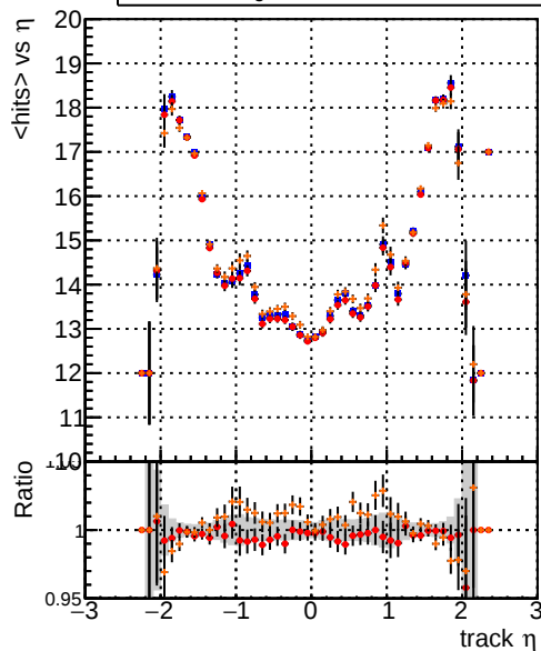
mean hits — DQM_TT_mkFit_ORIG — DQM_TT_mkFit_MODIF — /data2/legianni/newRel-PR129/sta/CMSSW_13_2_0_pre3/src/DQM_TT_MODIFok
