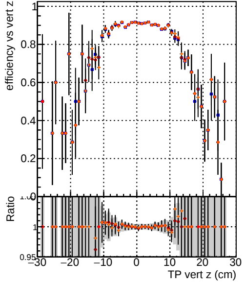
Efficiency vs. TP vert z —●— DQM_TT_mkFit_ORIG —●— DQM_TT_mkFit_MODIF —●— /data2/legianni/newRel-PR129/sta/CMSSW_13_2_0_pre3/src/DQM_TT_MODIFok
