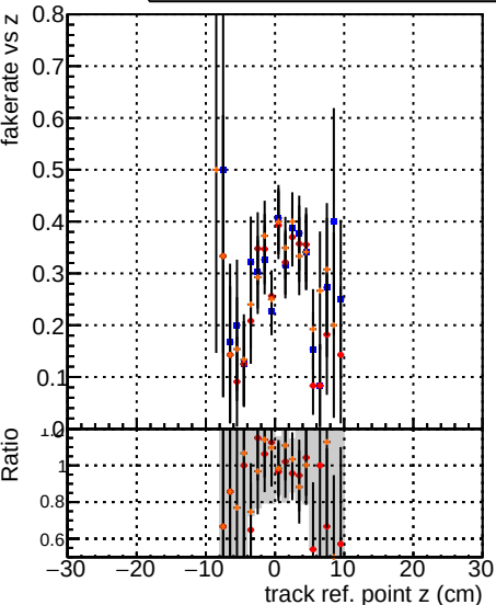
Fake rate vs verpos DQM TT mkFit ORIG DQM TT mkFit MODIF /data2/legianni/newRel-PR129/sta/CMSSW_13_2_0_pre3/src/DQM TT_MODIFok
