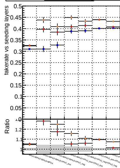
Fake rate vs. DOM TT mkFit ORIG DOM TT mkFit MODIE /data2/legianni/newRel-PR129/sta/CMSSW_13_2_0_pre3/src/DQM TT_MODIFok
