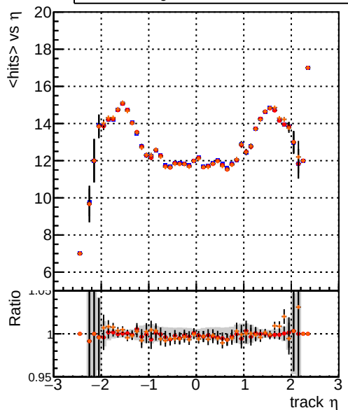
mean hits vs \eta — DQM_TT_mkFit_ORIG — DQM_TT_mkFit_MODIF — /data2/legianni/newRel-PR129/sta/CMSSW_13_2_0_pre3/src/DQM_TT_MODIFok
