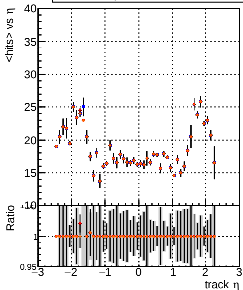
mean hits vs \eta Legend: DQM_TT_mkFit_ORIG (blue), DQM_TT_mkFit_MODIF (red), /data2/legianni/newRel-PR129/sta/CMSSW_13_2_0_pre3/src/DQM_TT_MODIFok (orange)
