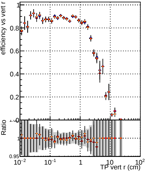
Efficiency vs TP vert r (cm) Legend: DQM_TT_mkFit_ORIG DQM_TT_mkFit_MODIF /data2/legianni/newRel-PR129/sta/CMSSW_13_2_0_pre3/src/DQM_TT_MODIFok
