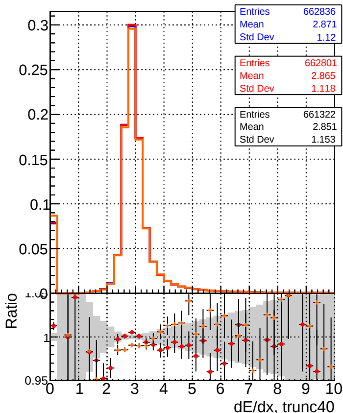
— DQM_TT_mkFit_ORIG — DQM_TT_mkFit_MODIF — /data2/legianni/newRel-PR129/sta/CMSSW_13_2_0_pre3/src/DQM_TT_MODIFok
