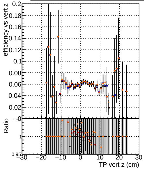
Efficiency vs. TP vert z (cm) — \bullet DQM TT mkFit ORIG — \bullet DQM TT mkFit MODIF — \bullet /data2/legianni/newRel-PR129/sta/CMSSW_13_2_0_pre3/src/DQM TT ORIGok — \bullet /data2/legianni/newRel-PR129/sta/CMSSW_13_2_0_pre3/src/DQM TT ORIG
