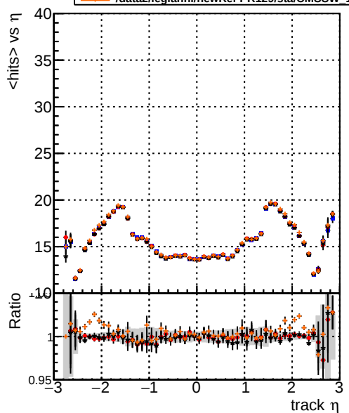
Legend: — DQM TT mkFit ORIG (blue line) — DQM TT mkFit MODIF (red line) — /data2/legianni/newRel-PR129/sta/CMSSW_13_2_0_pre3/src/DQM TT ORIGok (black line with dots) — /data2/legianni/newRel-PR129/sta/CMSSW_13_2_0_pre3/src/DQM TT ORIG (orange line)
