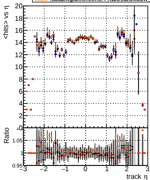
mean hits vs \eta — DQM TT mkFit ORIG — DQM TT mkFit MODIF — /data2/legianni/newRel-PR129/sta/CMSSW_13_2_0_pre3/src/DQM TT ORIG — /data2/legianni/newRel-PR129/sta/CMSSW_13_2_0_pre3/src/DQM TT MODIF
