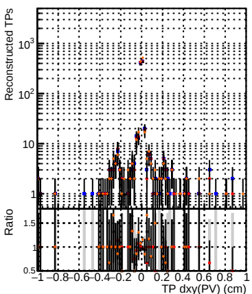
— DQM_TT_mkFit_ORIG — DQM_TT_mkFit_MODIF — /data2/legianni/newRel-PR129/sta/CMSSW_13_2_0_pre3/src/DQM_TT_ORIGok — /data2/legianni/newRel-PR129/sta/CMSSW_13_2_0_pre3/src/DQM_TT_ORIG
