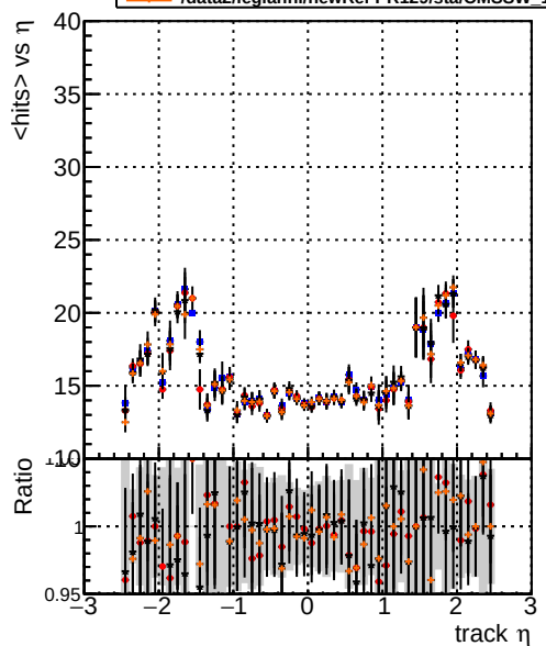
mean hits vs \eta DQM TT mkFit ORIG DQM TT mkFit MODIF /data2/legianni/newRel-PR129/sta/CMSSW_13_2_0_pre3/src/DQM TT_ORIGGok /data2/legianni/newRel-PR129/sta/CMSSW_13_2_0_pre3/src/DQM TT_ORIG
