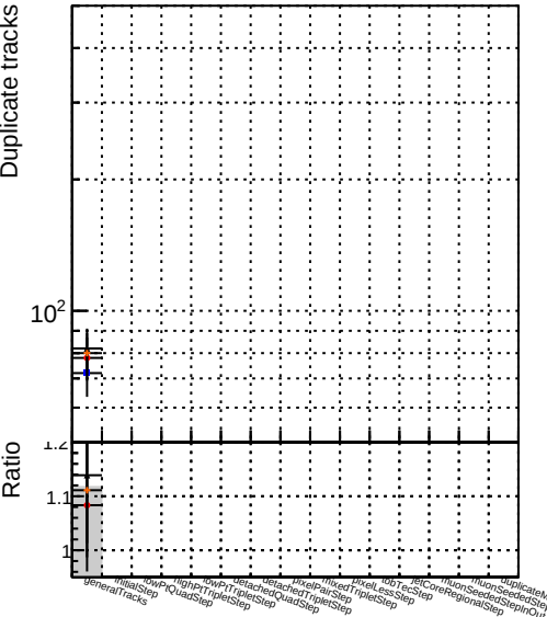
Number Path 1 /data2/legianni/newRel-PR129/sta/CMSSW_13_2_0_pre3/src/DQM_TT_ORIGOk 2 /data2/legianni/newRel-PR129/sta/CMSSW_13_2_0_pre3/src/DQM_TT_ORIG
