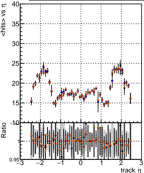
mean hit vs \eta — DQM TT mkFit ORIG — DQM TT mkFit MODIF — /data2/legianni/newRel-PR129/sta/CMSSW_13_2_0_pre3/src/DQM TT ORIGok — /data2/legianni/newRel-PR129/sta/CMSSW_13_2_0_pre3/src/DQM TT ORIG
