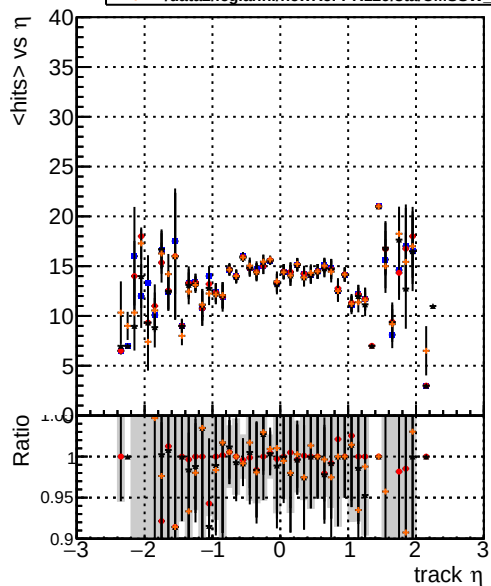
mean hits vs \eta — DQM TT mkFit ORIG — DQM TT mkFit MODIF — /data2/legianni/newRel-PR129/sta/CMSSW_13_2_0_pre3/src/DQM TT ORIGok — /data2/legianni/newRel-PR129/sta/CMSSW_13_2_0_pre3/src/DQM TT ORIG
