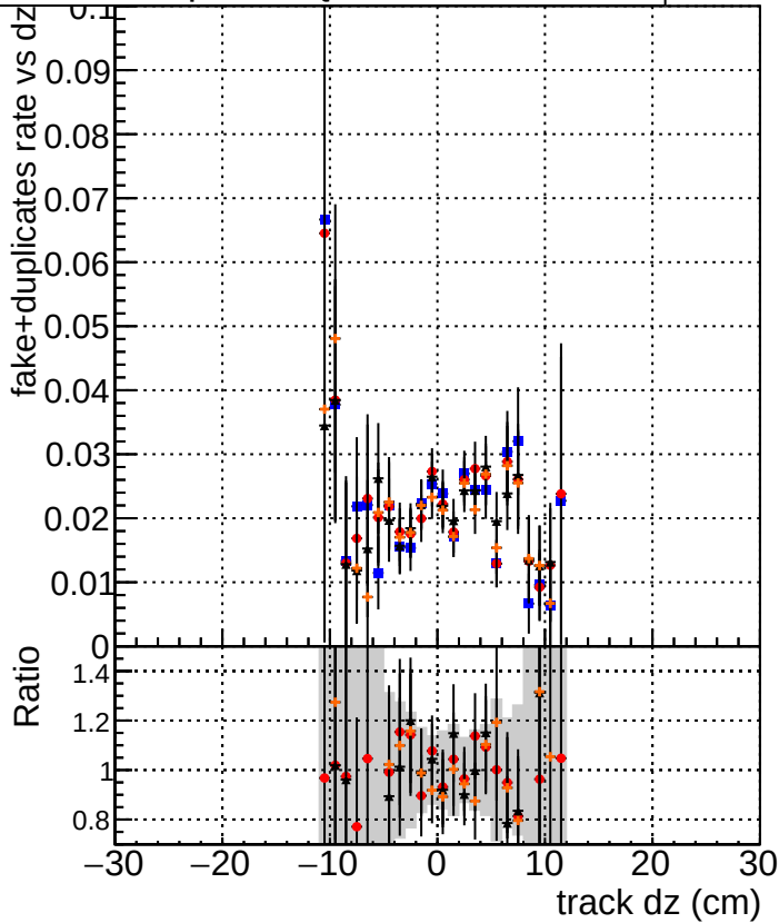
Legend for the bottom plot: DQM_TT_mkFit_ORIG DQM_TT_mkFit_MODIF /data2/legianni/newRel-PR129/sta/CMSSW_13_2_0_pre3/src/DQM_TT_ORIGOk /data2/legianni/newRel-PR129/sta/CMSSW_13_2_0_pre3/src/DQM_TT_ORIG
