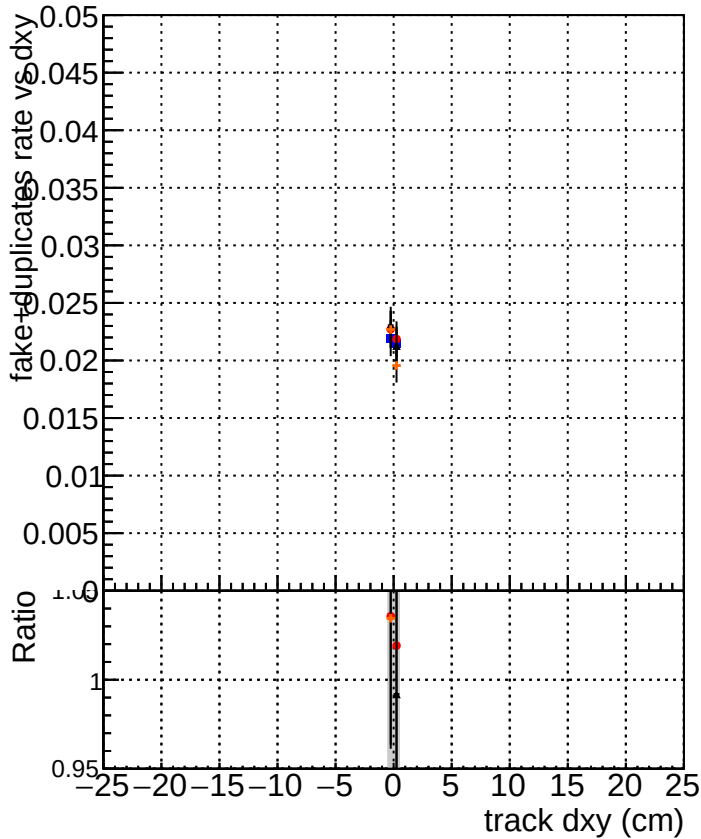
Legend for the bottom plot: DQM_TT_mkFit_ORIG DQM_TT_mkFit_MODIF /data2/legianni/newRel-PR129/sta/CMSSW_13_2_0_pre3/src/DQM_TT_ORIGOk /data2/legianni/newRel-PR129/sta/CMSSW_13_2_0_pre3/src/DQM_TT_ORIG
