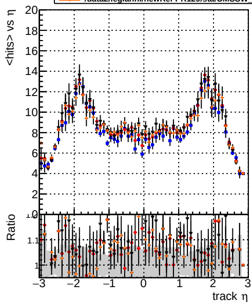
mean hits vs \eta Legend: blue line: DQM TT mkFit ORIG red line: DQM TT mkFit MODIF black line: /data2/legianni/newRel-PR129/sta/CMSSW_13_2_0_pre3/src/DQM TT_ORIGok orange line: /data2/legianni/newRel-PR129/sta/CMSSW_13_2_0_pre3/src/DQM TT_ORIG
