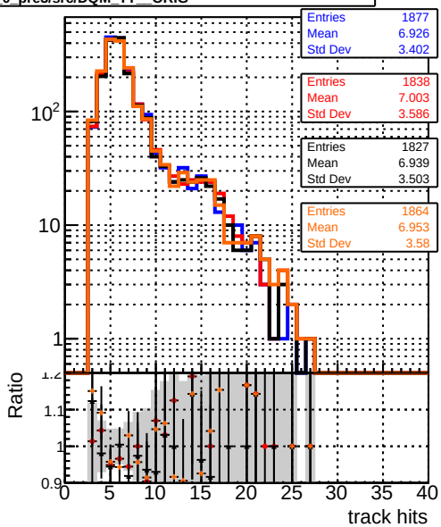
— DQM TT mkFit ORIG — DQM TT mkFit MODIF — /data2/legianni/newRel-PR129/sta/CMSSW_13_2_0_pre3/src/DQM TT_ORIGok — /data2/legianni/newRel-PR129/sta/CMSSW_13_2_0_pre3/src/DQM TT_ORIG
