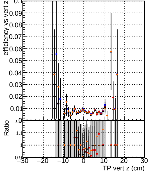
Efficiency vs vert z — DQM TT mkFit ORIG — DQM TT mkFit MODIF — /data2/legianni/newRel-PR129/sta/CMSSW_13_2_0_pre3/src/DQM TT ORIGok — /data2/legianni/newRel-PR129/sta/CMSSW_13_2_0_pre3/src/DQM TT ORIG
