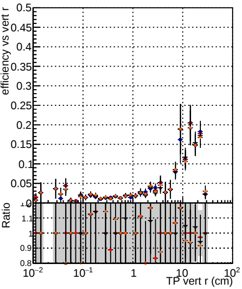
Efficiency vs vertpos Legend: — DQM_TT_mkFit_ORIG — DQM_TT_mkFit_MODIF — /data2/legianni/newRel-PR129/sta/CMSSW_13_2_0_pre3/src/DQM_TT_ORIGok — /data2/legianni/newRel-PR129/sta/CMSSW_13_2_0_pre3/src/DQM_TT_ORIG
