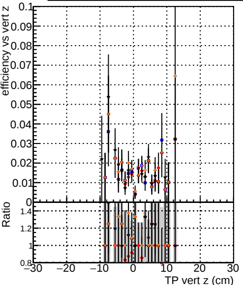
Efficiency vs vertpos Legend: DQM_TT_mkFit_ORIG DQM_TT_mkFit_MODIF /data2/legianni/newRel-PR129/sta/CMSSW_13_2_0_pre3/src/DQM_TT_ORIGok /data2/legianni/newRel-PR129/sta/CMSSW_13_2_0_pre3/src/DQM_TT_ORIG
