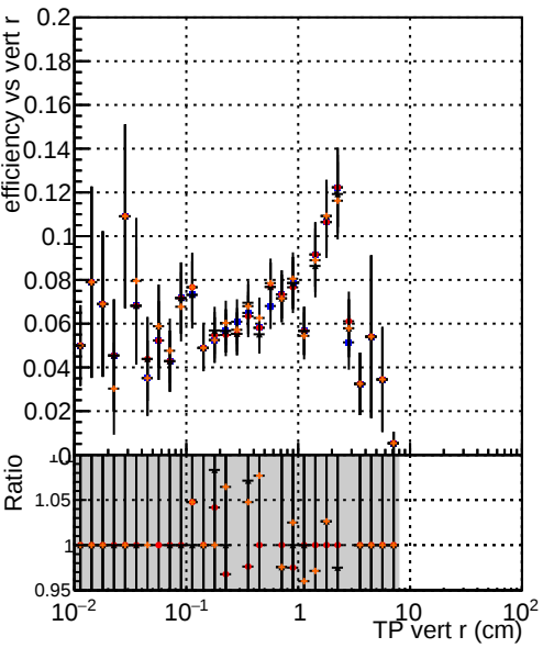
Efficiency vs vertpos Legend: —•— DQM_TT_mkFit_ORIG —•— DQM_TT_mkFit_MODIF —•— /data2/legianni/newRel-PR129/sta/CMSSW_13_2_0_pre3/src/DQM_TT_ORIGok —•— /data2/legianni/newRel-PR129/sta/CMSSW_13_2_0_pre3/src/DQM_TT_ORIG
