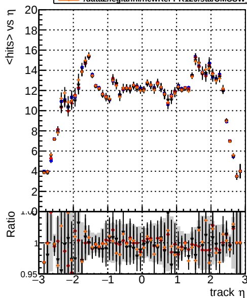
mean hits — DQM TT mkFit ORIG — DQM TT mkFit MODIF — /data2/legianni/newRel-PR129/sta/CMSSW_13_2_0_pre3/src/DQM TT_ORIGok — /data2/legianni/newRel-PR129/sta/CMSSW_13_2_0_pre3/src/DQM TT_ORIG
