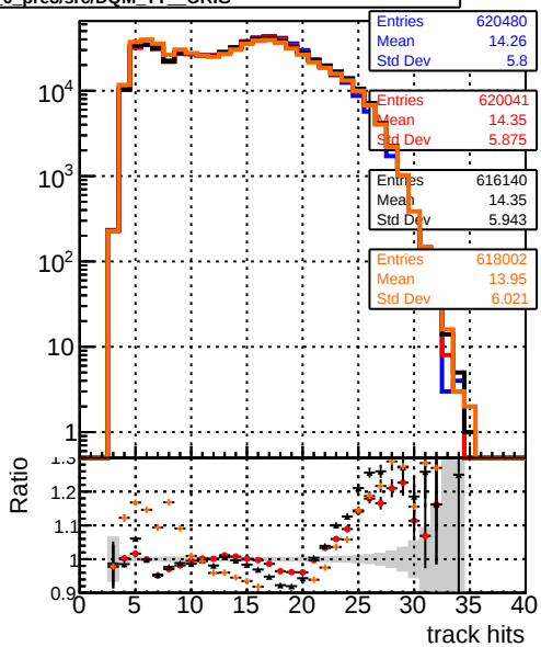
Legend: — DQM TT mkFit ORIG (blue line) — DQM TT mkFit MODIF (red line) — /data2/legianni/newRel-PR129/sta/CMSSW_13_2_0_pre3/src/DQM TT_ORIGok (black line) — /data2/legianni/newRel-PR129/sta/CMSSW_13_2_0_pre3/src/DQM TT_ORIG (orange line)
