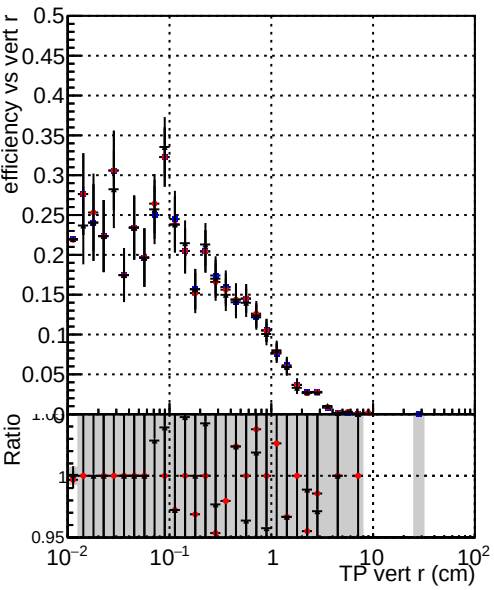
Efficiency vs vertpos Legend: DQM_TT_mkFit_ORIG DQM_TT_mkFit_MODIF data2/legianni/newRel-PR129/sta/CMSSW_13_2_0_pre3/src/DQM_TT_ORIG
