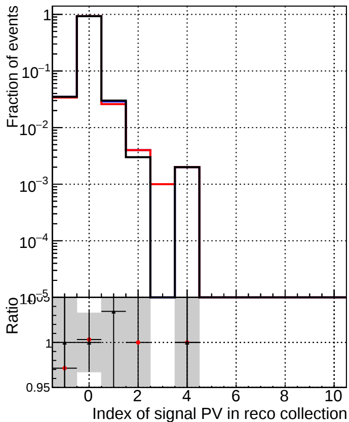
—■ DQM_TT_mkFit_ORIG —● DQM_TT_mkFit_MODIF —■ /data2/legianni/newRel-PR129/sta/CMSSW_13_2_0_pre3/src/DQM_TT_ORIG
