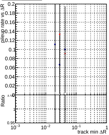
Legend: DQM TT mkFit ORIG (blue dots), DQM TT mkFit MODIF (red dots), /data2/legianni/newRel-PR129/sta/CMSSW_13_2_0_pre3/src/DQM_TT_ORIG (grey shaded area)
