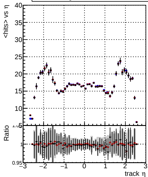
mean hits — DQM_TT_mkFit_ORIG — DQM_TT_mkFit_MODIF — /data2/legianni/newRel-PR129/sta/CMSSW_13_2_0_pre3/src/DQM_TT_ORIG
