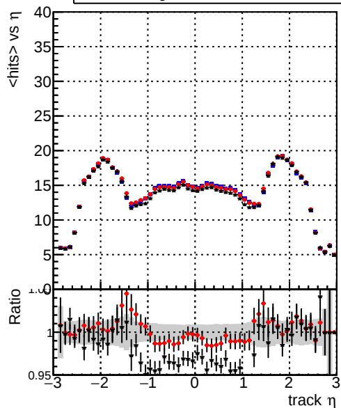
mean hits vs \eta — DQM_TT_mkFit_ORIG — DQM_TT_mkFit_MODIF — /data2/legianni/newRel-PR129/sta/CMSSW_13_2_0_pre3/src/DQM_TT_ORIG
