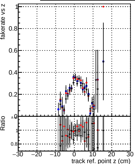
Legend: DQM TT mkFit ORIG (blue circles), DQM TT mkFit MODIF (red circles), /data2/legianni/newRel-PR129/sta/CMSSW_13_2_0_pre3/src/DQM TT_ORIG (black circles)
