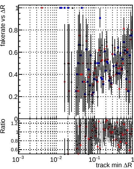
Legend: DQM TT mkFit ORIG (blue dots), DQM TT mkFit MODIF (red dots), /data2/legianni/newRel-CMSSW_13_2_0_pre3/src/DQM_TT_ORIG (black line with error bars)
