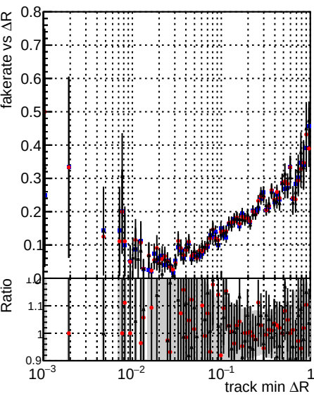
Legend: DQM TT mkFit ORIG (black circles), DQM TT mkFit MODIF (red circles), /data2/legianni/newRel-PR129/sta/CMSSW_13_2_0_pre3/src/DQM TT ORIG (black circles with error bars)
