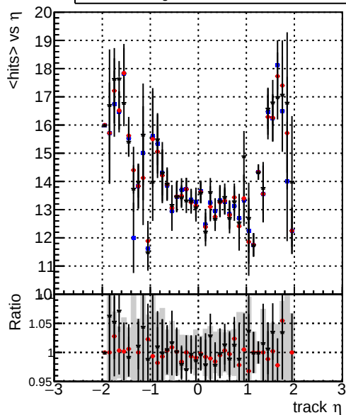
mean hit — DQM_TT_mkFit_ORIG — DQM_TT_mkFit_MODIF — /data2/legianni/newRel-PR129/sta/CMSSW_13_2_0_pre3/src/DQM_TT_ORIG
