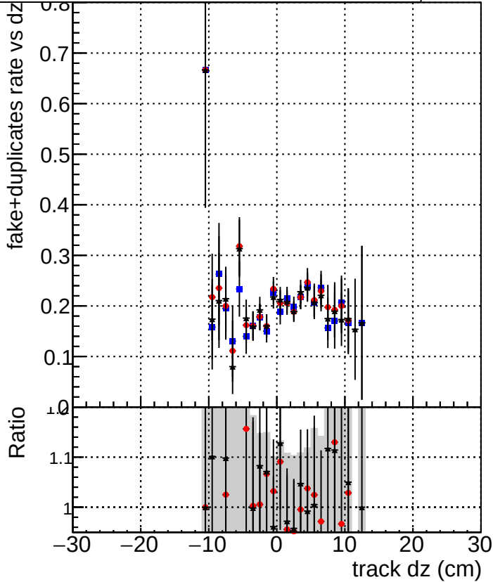
Legend: ■ DQM TT mkFit ORIG ● DQM TT mkFit MODIF ▲ /data2/legianni/newRel-PR129/sta/CMSSW_13_2_0_pre3/src/DQM_TT_ORIG
