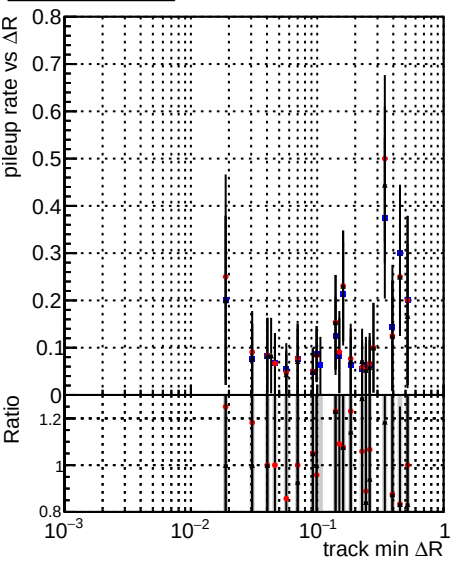
Legend: DQM TT mkFit ORIG (blue dots), DQM TT mkFit MODIF (red dots), /data2/legianni/newRel-PR129/sta/CMSSW_13_2_0_pre3/src/DQM TT_ORIG (black dots with error bars)
