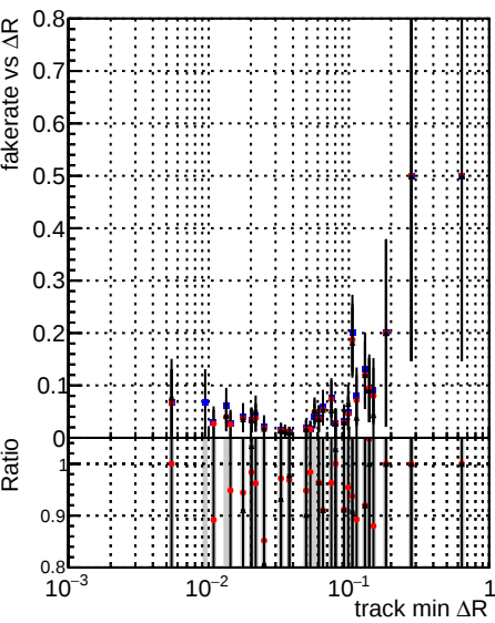
Fake rate vs \Delta R(\text{track, jet}) DQM TT mkFit ORIG DQM TT mkFit MODIF /data2/legianni/newRel-PR129/sta/CMSSW_13_2_0_pre3/src/DQM_TT_ORIG
