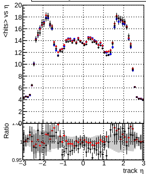
mean hit — DQM_TT_mkFit_ORIG — DQM_TT_mkFit_MODIF — /data2/legianni/newRel-PR129/sta/CMSSW_13_2_0_pre3/src/DQM_TT_ORIG
