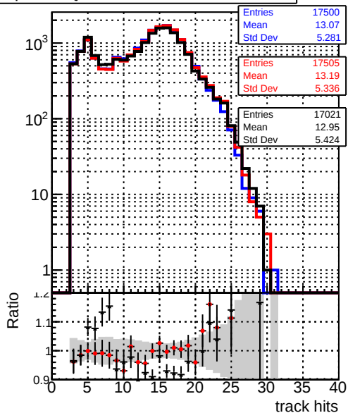
mean hit — DQM_TT_mkFit_ORIG — DQM_TT_mkFit_MODIF — /data2/legianni/newRel-PR129/sta/CMSSW_13_2_0_pre3/src/DQM_TT_ORIG
