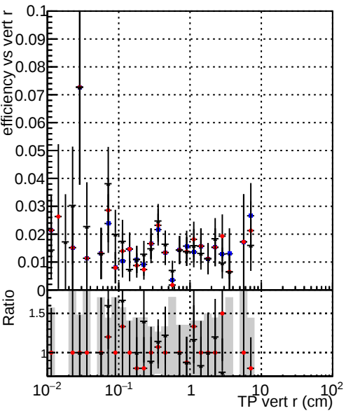
Efficiency vs TP vert r (cm) Legend: DQM_TT_mkFit_ORIG DQM_TT_mkFit_MODIF /data2/legianni/newRel-PR129/sta/CMSSW_13_2_0_pre3/src/DQM_TT_ORIG
