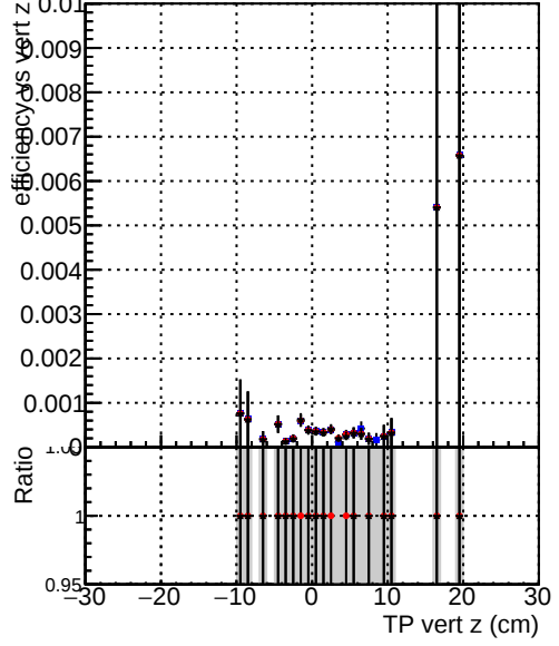
Efficiency vs TP vert z Legend: DQM_TT_mkFit_ORIG (blue line with circles) DQM_TT_mkFit_MODIF (red line with circles) /data2/legianni/newRel-PR129/sta/CMSSW_13_2_0_pre3/src/DQM_TT_ORIG (black line with circles)
