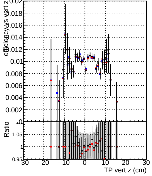
Efficiency vs. TP vert z — DQM_TT_mkFit_ORIG — DQM_TT_mkFit_MODIF — data2/legianni/newRel-PR129/sta/CMSSW_13_2_0_pre3/src/DQM_TT_ORIG
