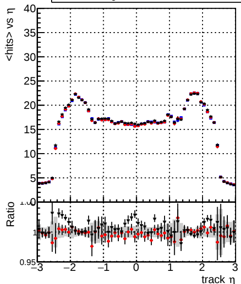
DQM_TT_mkFit_ORIG DQM_TT_mkFit_MODIF /data2/legianni/newRel-PR129/sta/CMSSW_13_2_0_pre3/src/DQM_TT_ORIG mean hits
