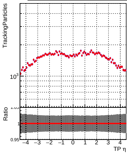
N of simulated tracks vs \eta Legend: —•— DQM_beforePR —•— DQM_correctCheck
