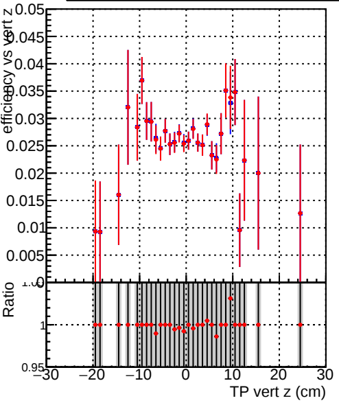
Efficiency vs TP vert z (cm) Legend: DQM_beforePR (blue line with markers), DQM_correctCheck (red line with markers)
