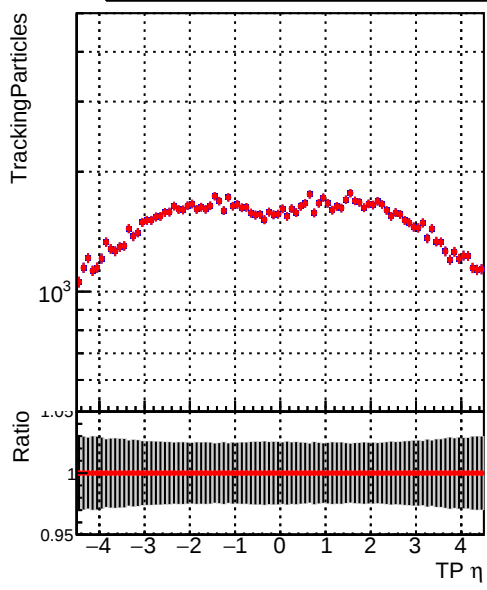
N of simulated tracks vs \eta Legend: DQM_beforePR (blue line with dots), DQM_correctCheck (red line with dots)
