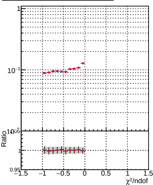
PackedCandidate::bestTrack() - reco::Track in normalizedChi2Q
